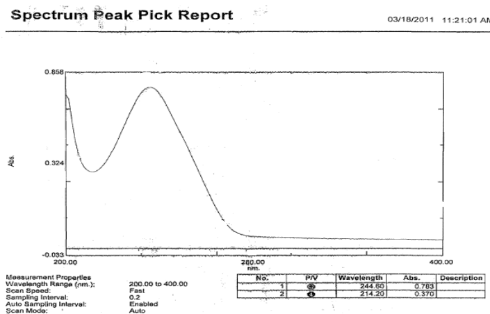
Figure 4: UV spectrum of API-1 in 0.1N HCl.
