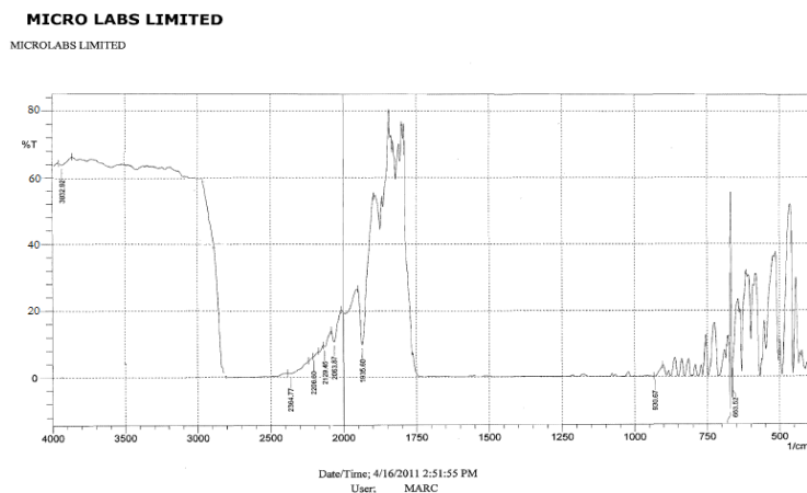
Figure 7: FT-IR spectrum of API-2.
