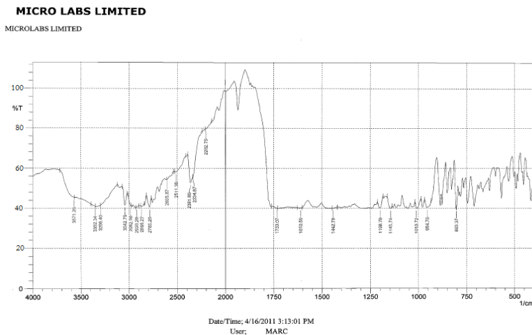
Figure 10: FT-IR spectrum of API-1 + API-2 + Povidone K-30.
