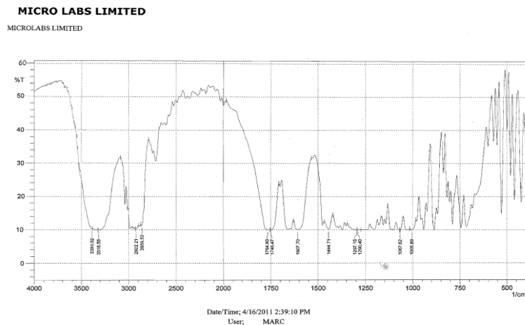
Figure 6: FT-IR spectrum of API-1.
