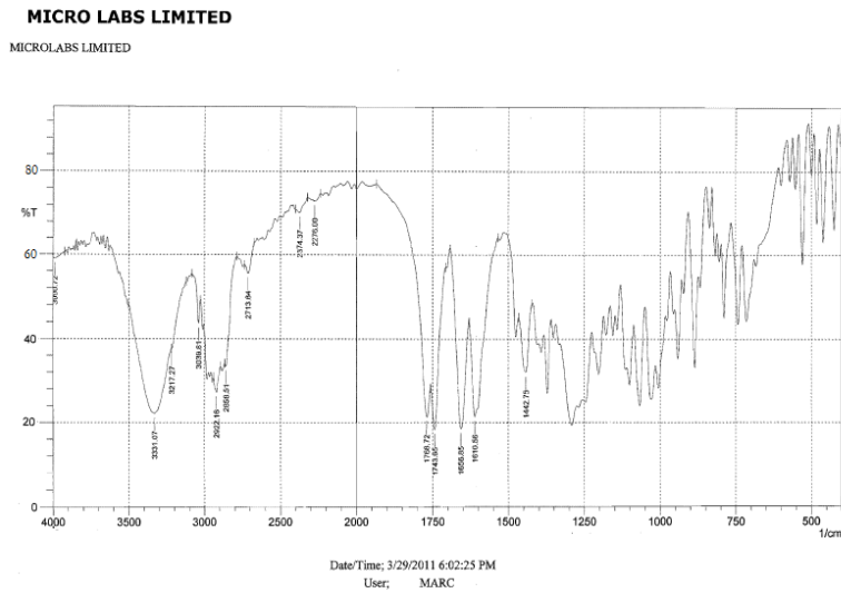
Figure 8: FT-IR spectrum of API-1 + API-2 combination.
