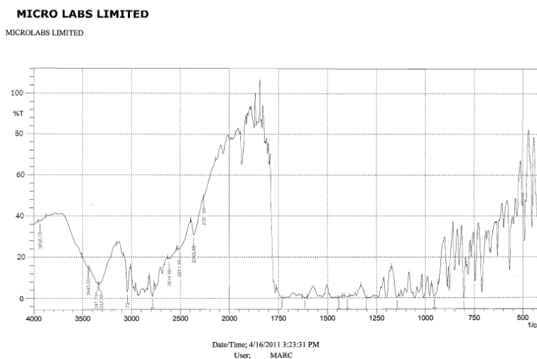
Figure 12: FT-IR spectrum of API-1 + API-2 + Trisodium citrate.
