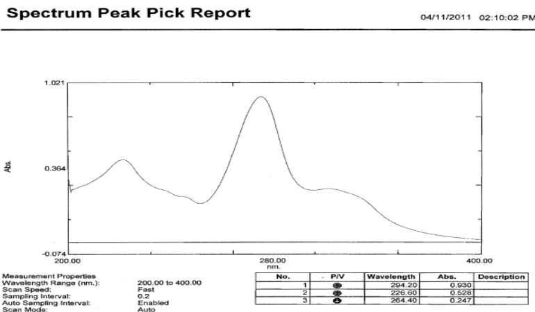
Figure 5: UV spectrum of API-2 in 0.1N HCl.
