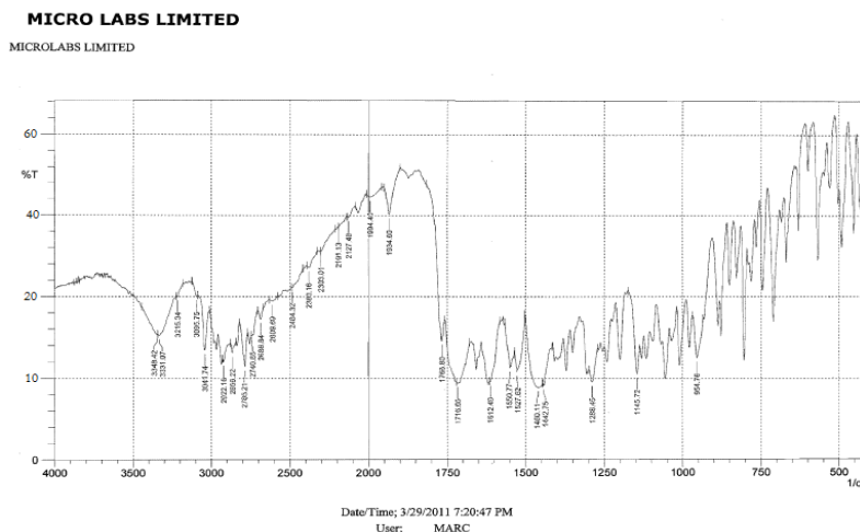
Figure 11: FT-IR spectrum of API-1 + API-2 + Citric acid.
