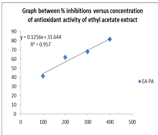
Figure 5.2 Graph between % inhibitions versus concentration of antioxidant activity of ethyl acetate extract.
