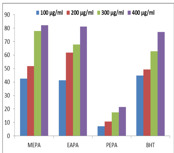
Figure 5.4: Comparative antioxidant study of P. articulata extract fractions with BHT.
